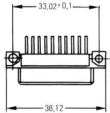
Bauform R/3 max. 30polig
